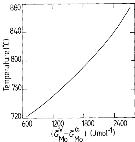
Figure 2 Plot of the difference (\bar{G}_{Mo}^{\gamma} - \bar{G}_{Mo}^{\alpha}) in partial molar free energy of molybdenum in austenite and in ferrite, assuming that the compositions of these two phases is that obtained at the interface during paraequilibrium transformation, as a function of transformation temperature. See text for detailed explanation.
